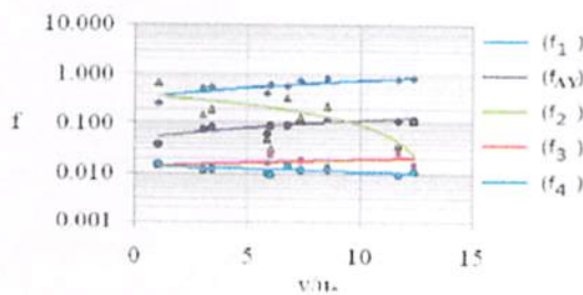
Figure 10. Friction factor vs v/u^* ratio at third research location
