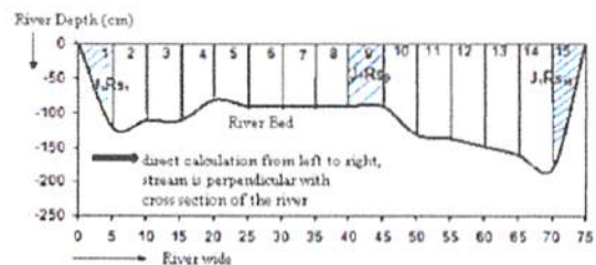
Figure 2. The cross section area and its guide line placed the bed load apparatus and other measurements
