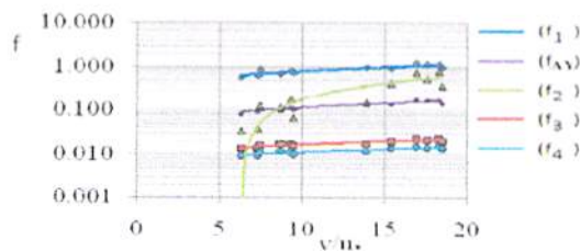
Figure 11. Friction factor vs v/u^* ratio at fourth research location
