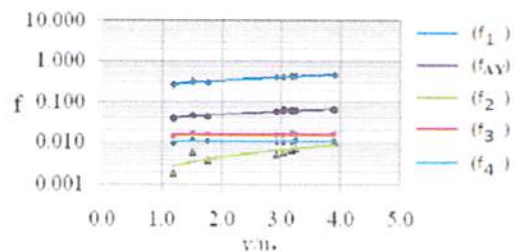
Figure 8. Friction factor vs v/u_* ratio at first research location
